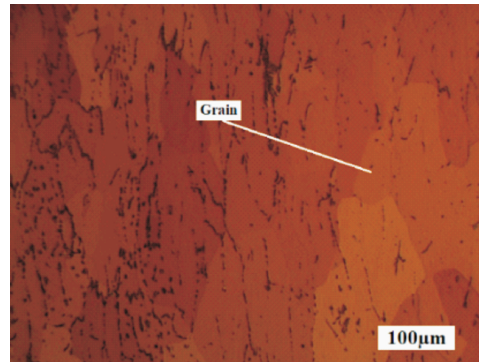
Fig. 5. AA 6061 + 3% NiCr in the presence of TiC
