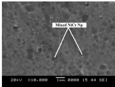
Fig. 4. AA-6061 + 6% NiCr in the presence of TiC
