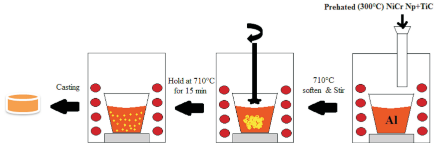
Fig. 1. Molten Aluminium in-situ technique
