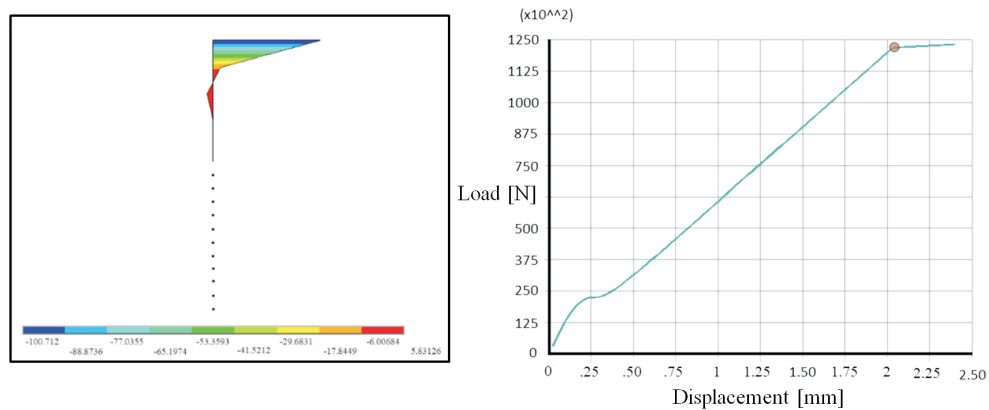
Fig. 5. Typical normal stresses diagram in the process zone and the beam force-displacement curve
