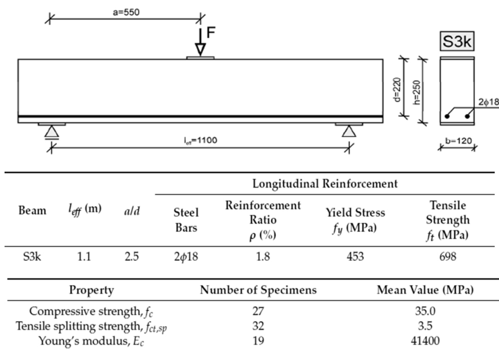
Fig. 3. Test model of the beam
