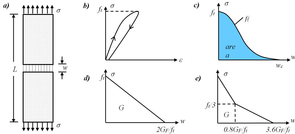
Fig. 1. Hillerborg's theory (a) concrete element on tension, (b) \sigma - \varepsilon diagram out of the fracture zone, (c) (\sigma - w) diagram in the fracture zone (d) and (e) numerical modelling of the (\sigma - w) diagram
