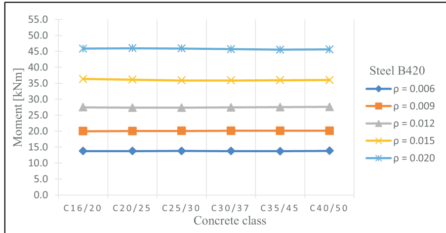
Fig. 6. Bending moment-concrete class for steel B420
