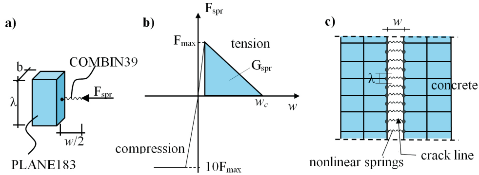
Fig. 2. Nonlinear springs (a) spring's zone, (b) linear spring model, (c) FE model
