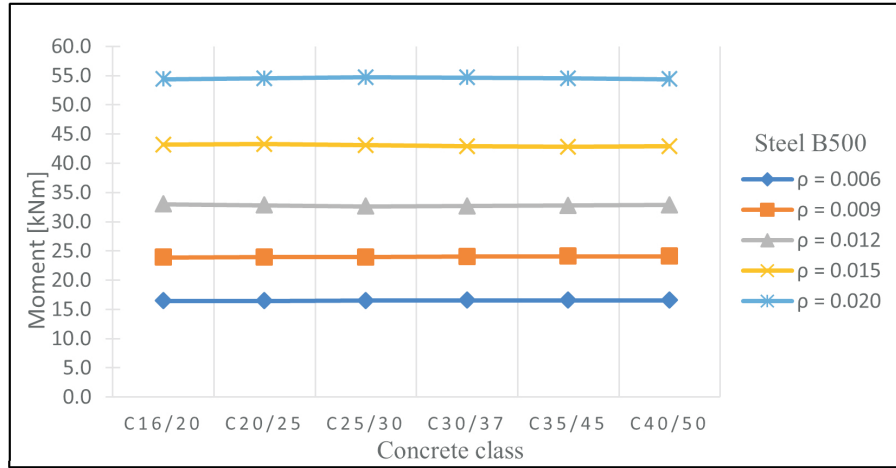
Fig. 8. Bending moment-concrete class for steel B500
