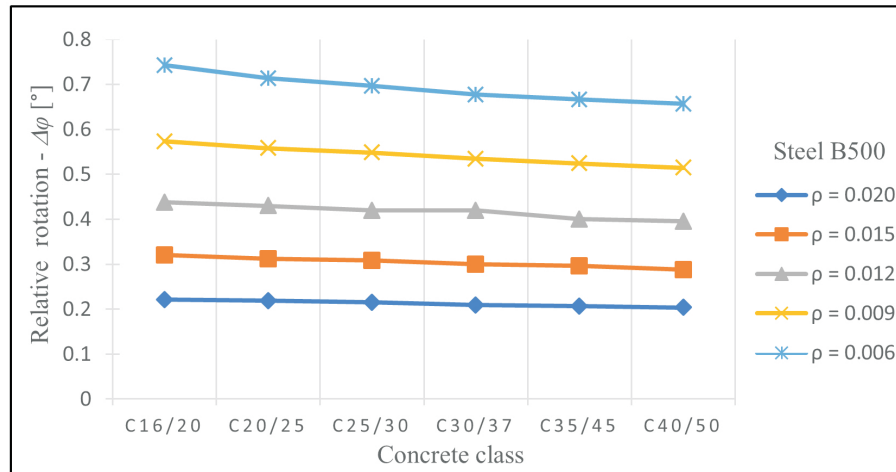
Fig. 9. Relative rotation-concrete class for steel B500
