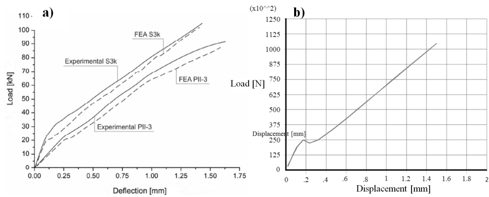
Fig. 4. Load-displacement curves for test beam S3k: a) results from [3]; b) results from presented model
