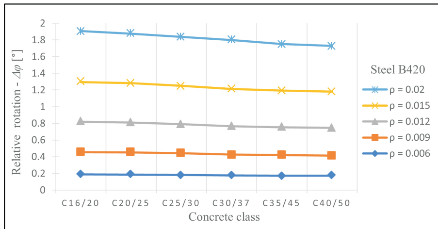
Fig. 7. Relative rotation-concrete class for steel B420
